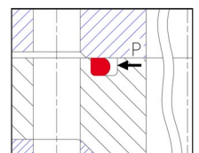
O-ring deformed under pressure
